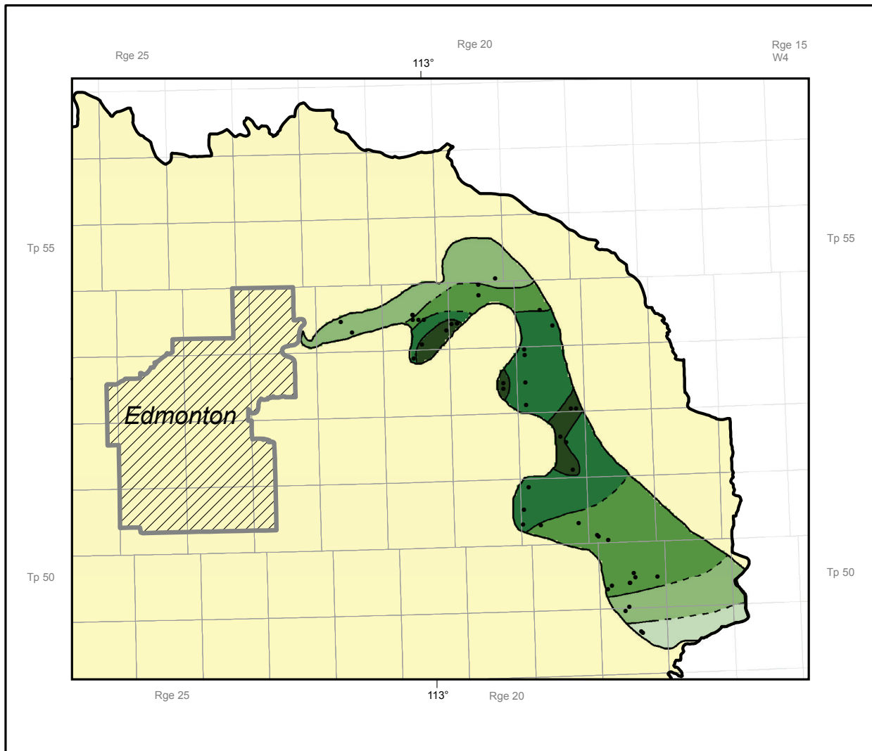
Figure 9. Ranges of alkalinity as calcium carbonate in fresh groundwater in the Bearpaw aquifer.
