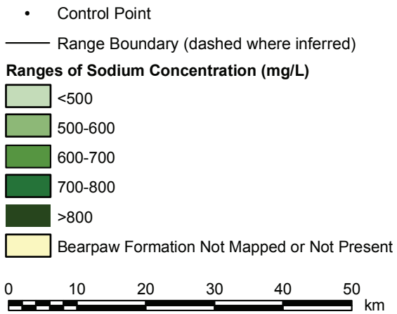
Figure 5. Ranges of sodium concentration in fresh groundwater in the Bearpaw aquifer.
