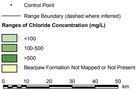
Figure 7. Ranges of chloride concentration in fresh groundwater in the Bearpaw aquifer.
