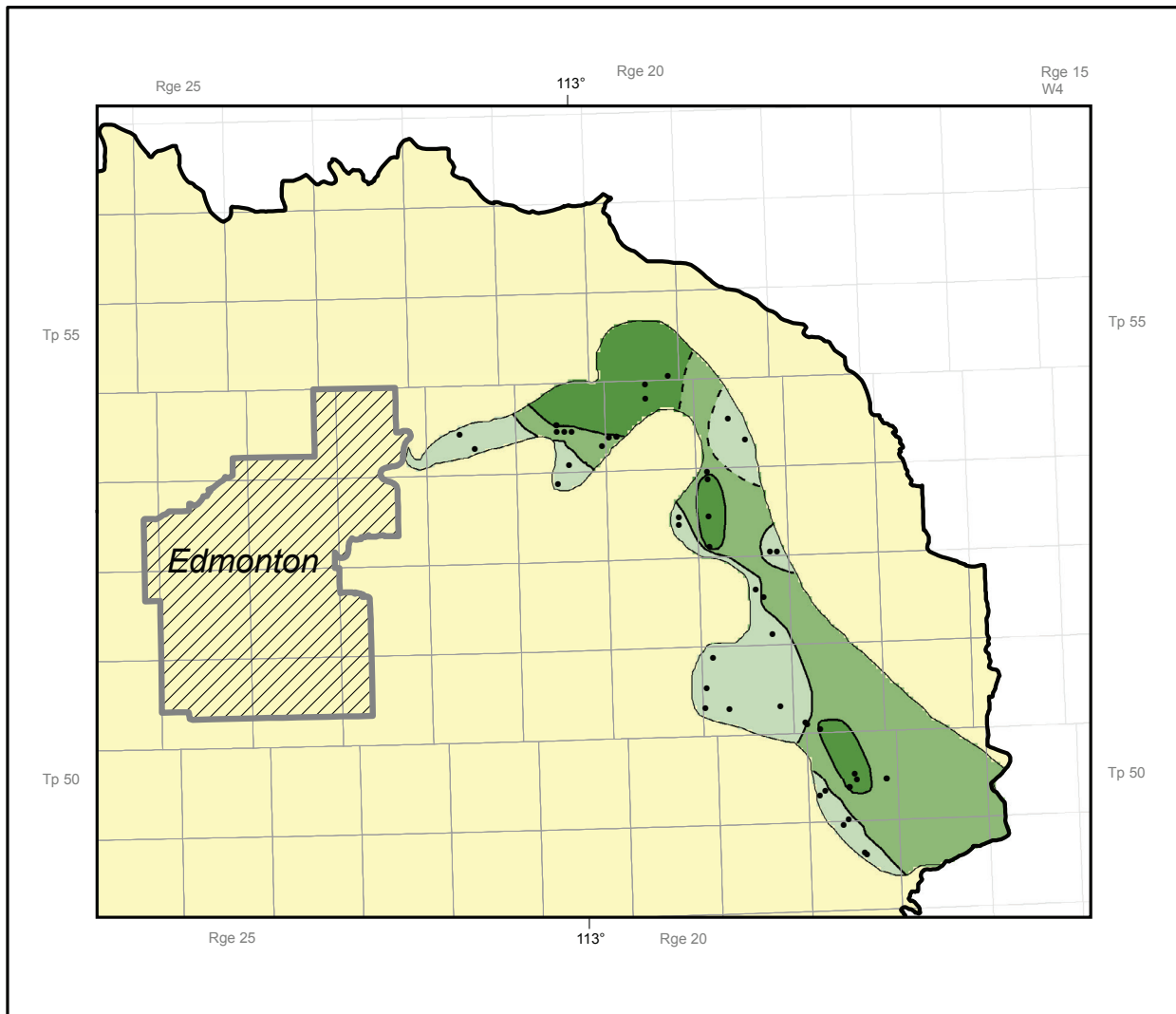
Figure 3. Ranges of calcium concentration in fresh groundwater in the Bearpaw aquifer.
