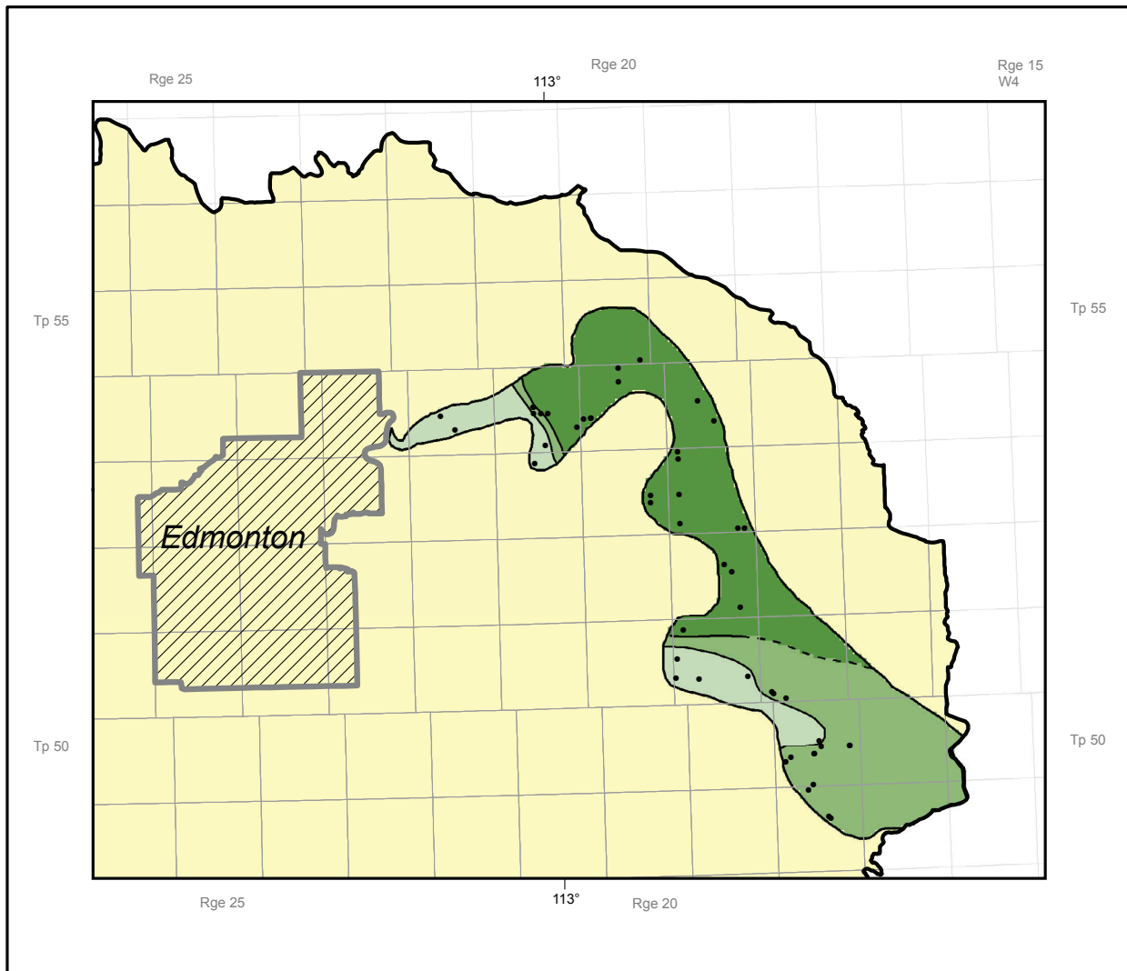
Figure 6. Ranges of potassium concentration in fresh groundwater in the Bearpaw aquifer.
