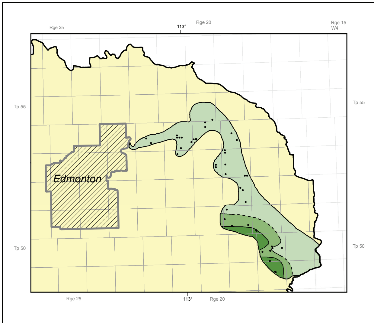
Figure 7. Ranges of chloride concentration in fresh groundwater in the Bearpaw aquifer.
