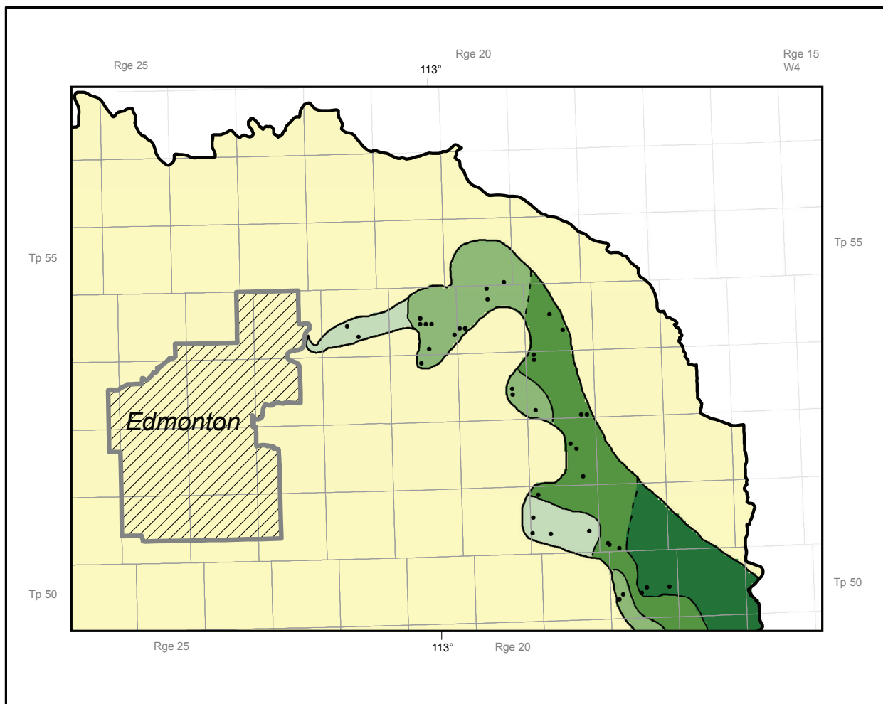
Figure 8. Ranges of sulphate concentration in fresh groundwater in the Bearpaw aquifer.
