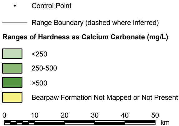
Figure 12. Ranges of hardness as calcium carbonate in fresh groundwater in the Bearpaw aquifer.
