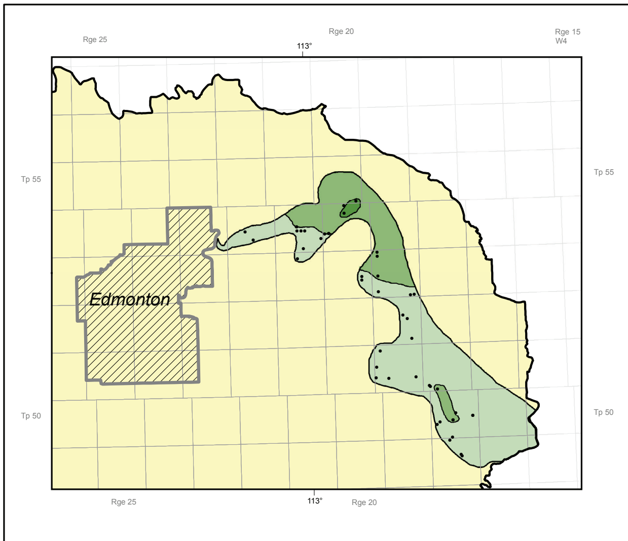
Figure 12. Ranges of hardness as calcium carbonate in fresh groundwater in the Bearpaw aquifer.
