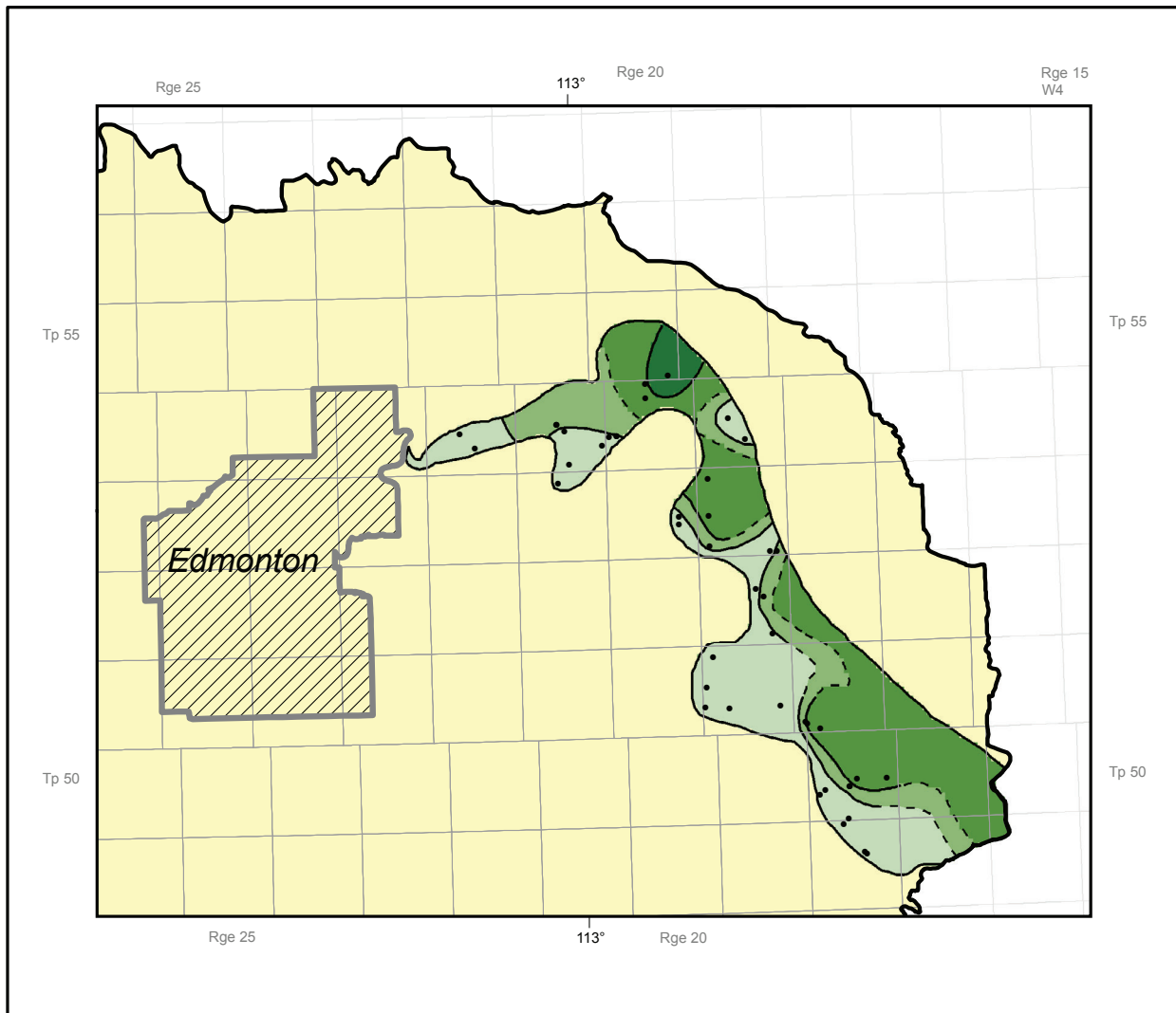
Figure 4. Ranges of magnesium concentration in fresh groundwater in the Bearpaw aquifer.
