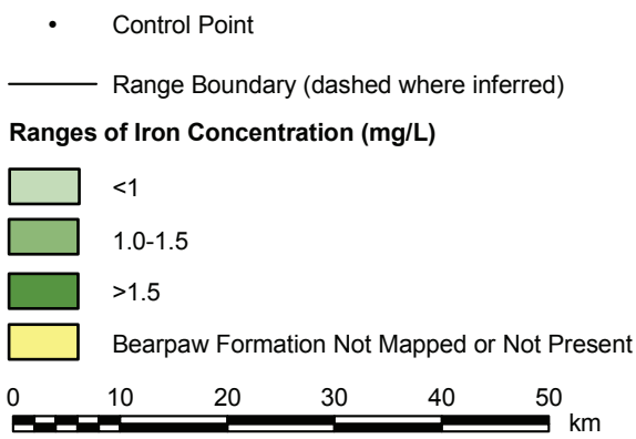
Figure 10. Ranges of iron concentration in fresh groundwater in the Bearpaw aquifer.
