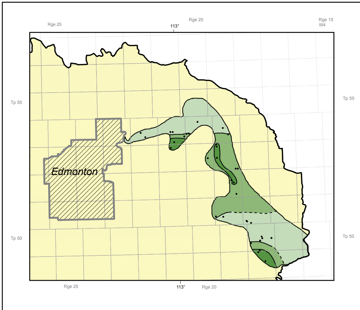
Figure 10. Ranges of iron concentration in fresh groundwater in the Bearpaw aquifer.
