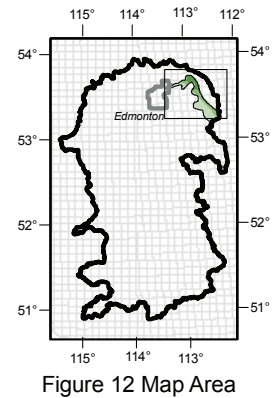
Figure 12. Ranges of hardness as calcium carbonate in fresh groundwater in the Bearpaw aquifer.
