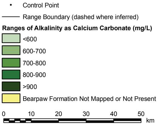
Figure 9. Ranges of alkalinity as calcium carbonate in fresh groundwater in the Bearpaw aquifer.
