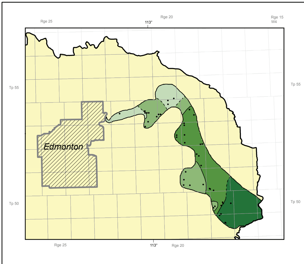
Figure 11. Ranges of total dissolved solids concentration in fresh groundwater in the Bearpaw aquifer.
