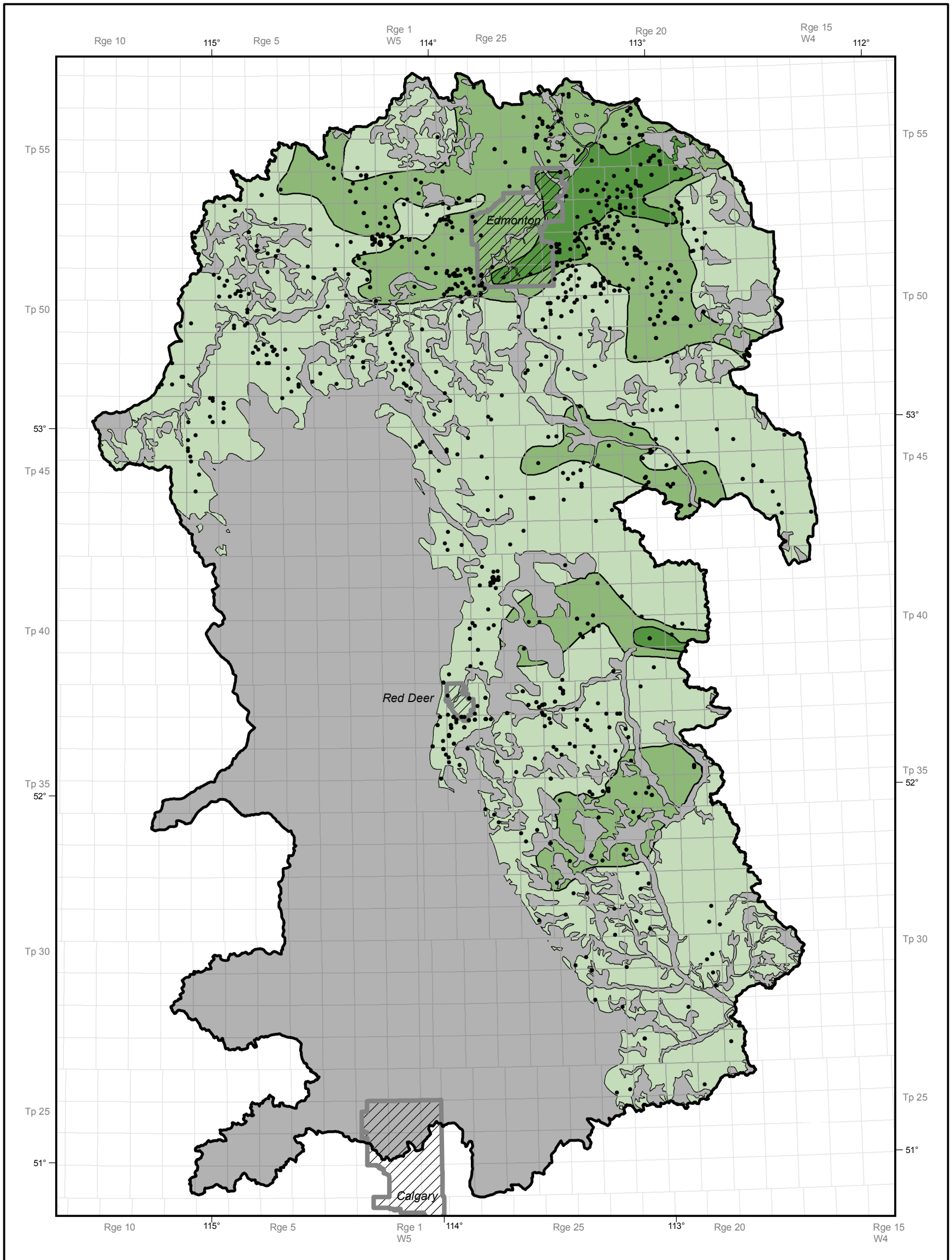
Figure 12. Ranges of hardness as calcium carbonate in fresh groundwater in the surficial sediments aquifer.
