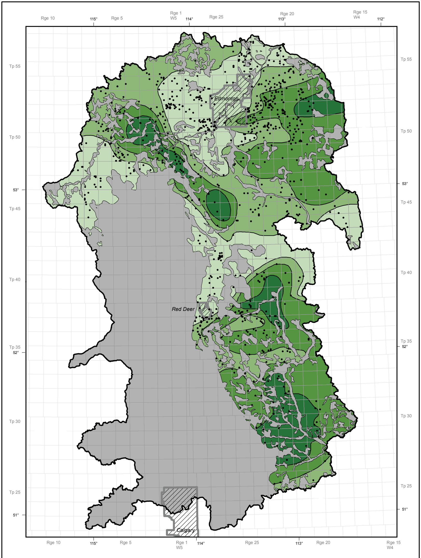
Figure 9. Ranges of alkalinity as calcium carbonate in fresh groundwater in the surficial sediments aquifer.
