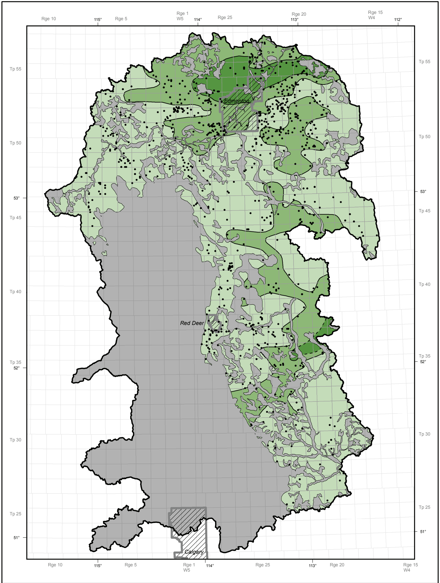
Figure 3. Ranges of calcium concentration in fresh groundwater in the surficial sediments aquifer.
