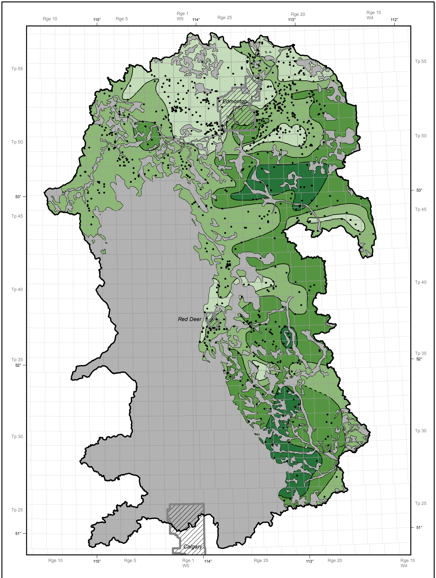
Figure 5. Ranges of sodium concentration in fresh groundwater in the surficial sediments aquifer.
