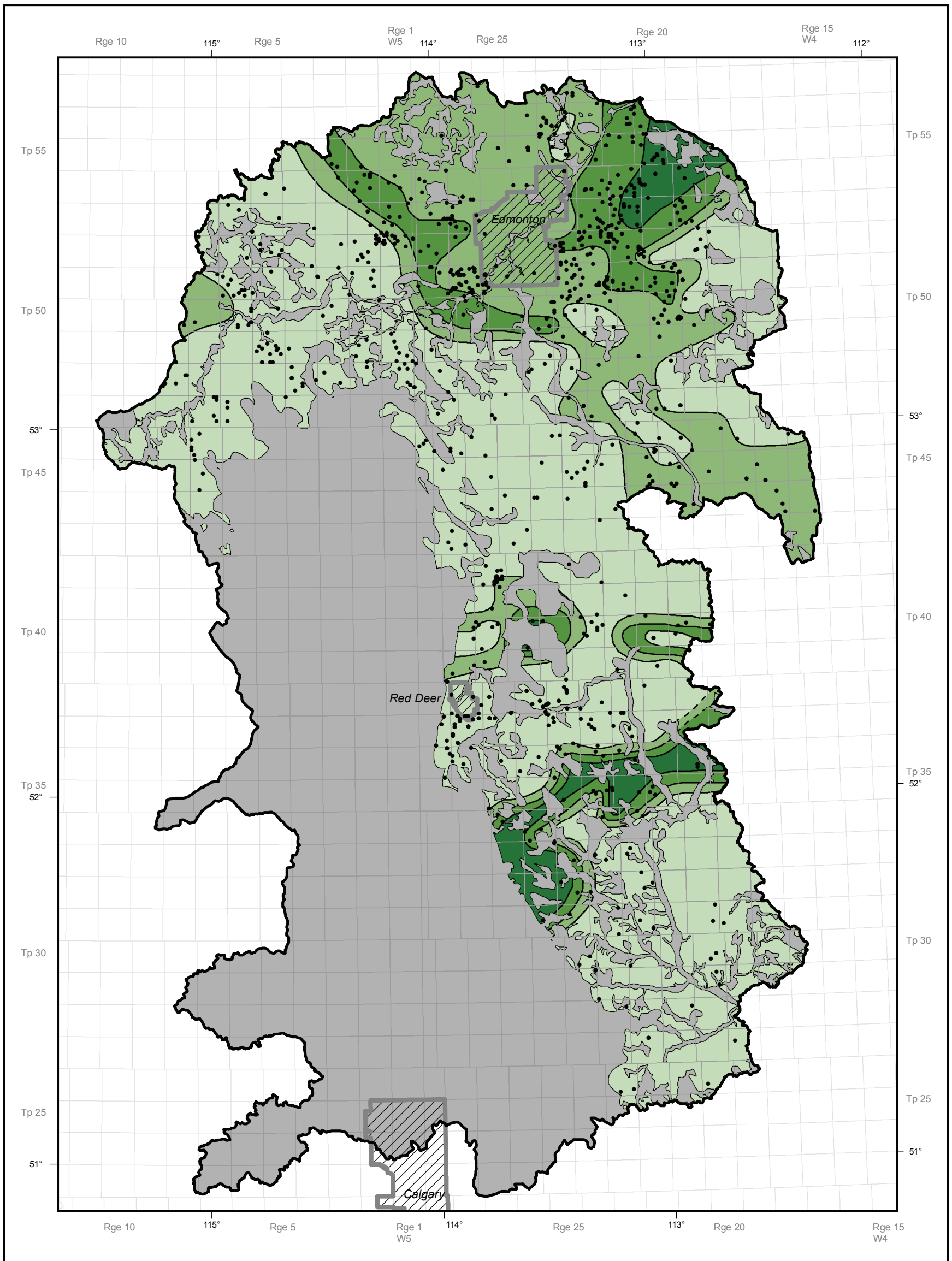
Figure 4. Ranges of magnesium concentration in fresh groundwater in the surficial sediments aquifer.
