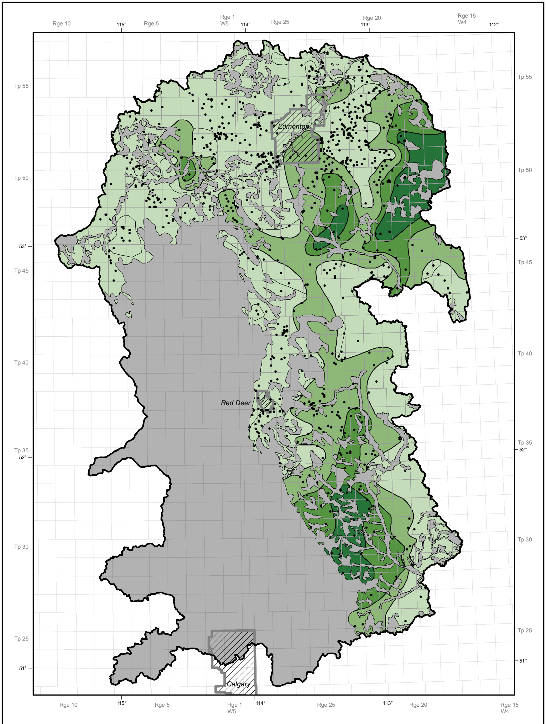
Figure 11. Ranges of total dissolved solids concentration in fresh groundwater in the surficial sediments aquifer.
