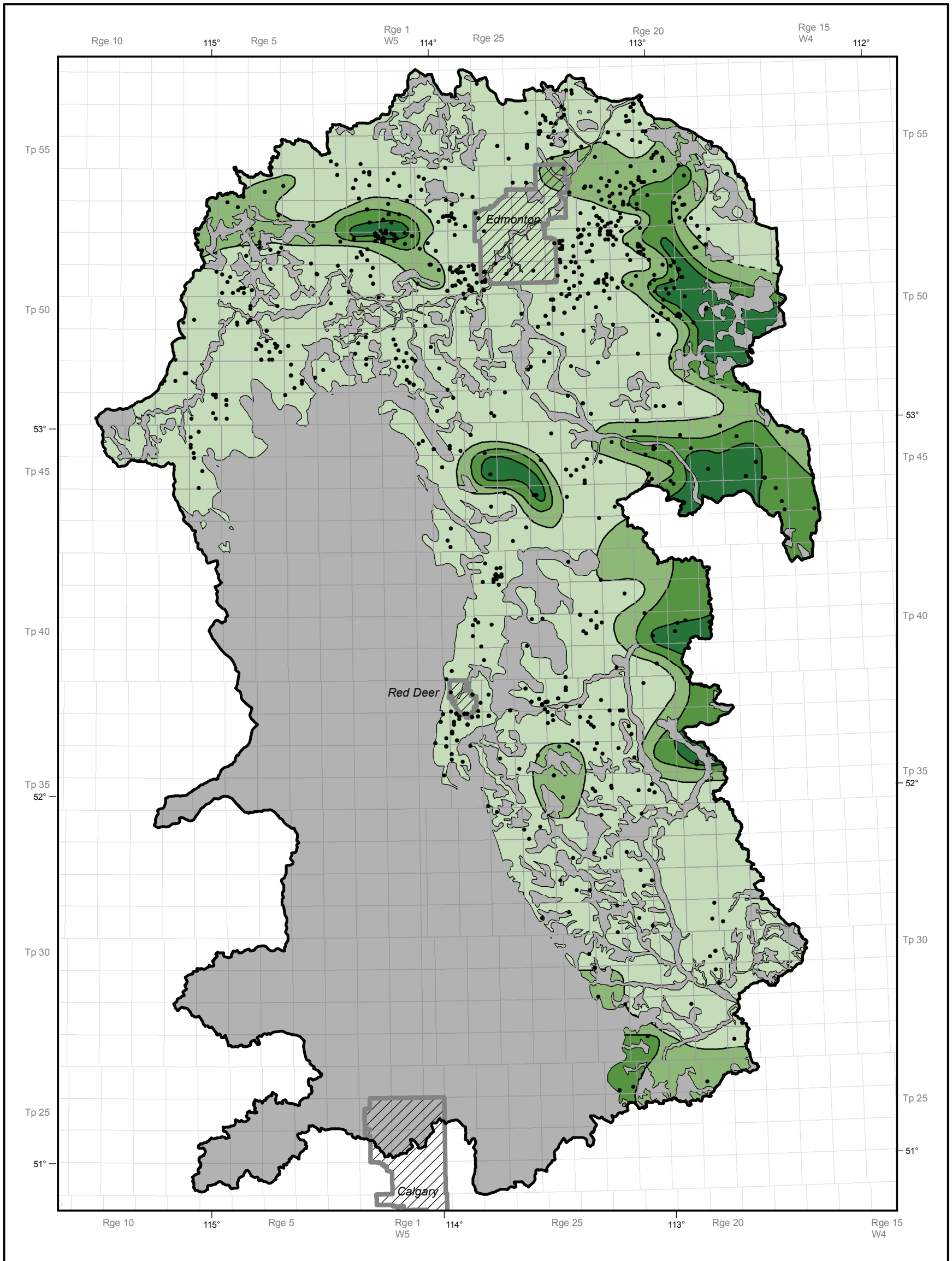
Figure 10. Ranges of iron concentration in fresh groundwater in the surficial sediments aquifer.
