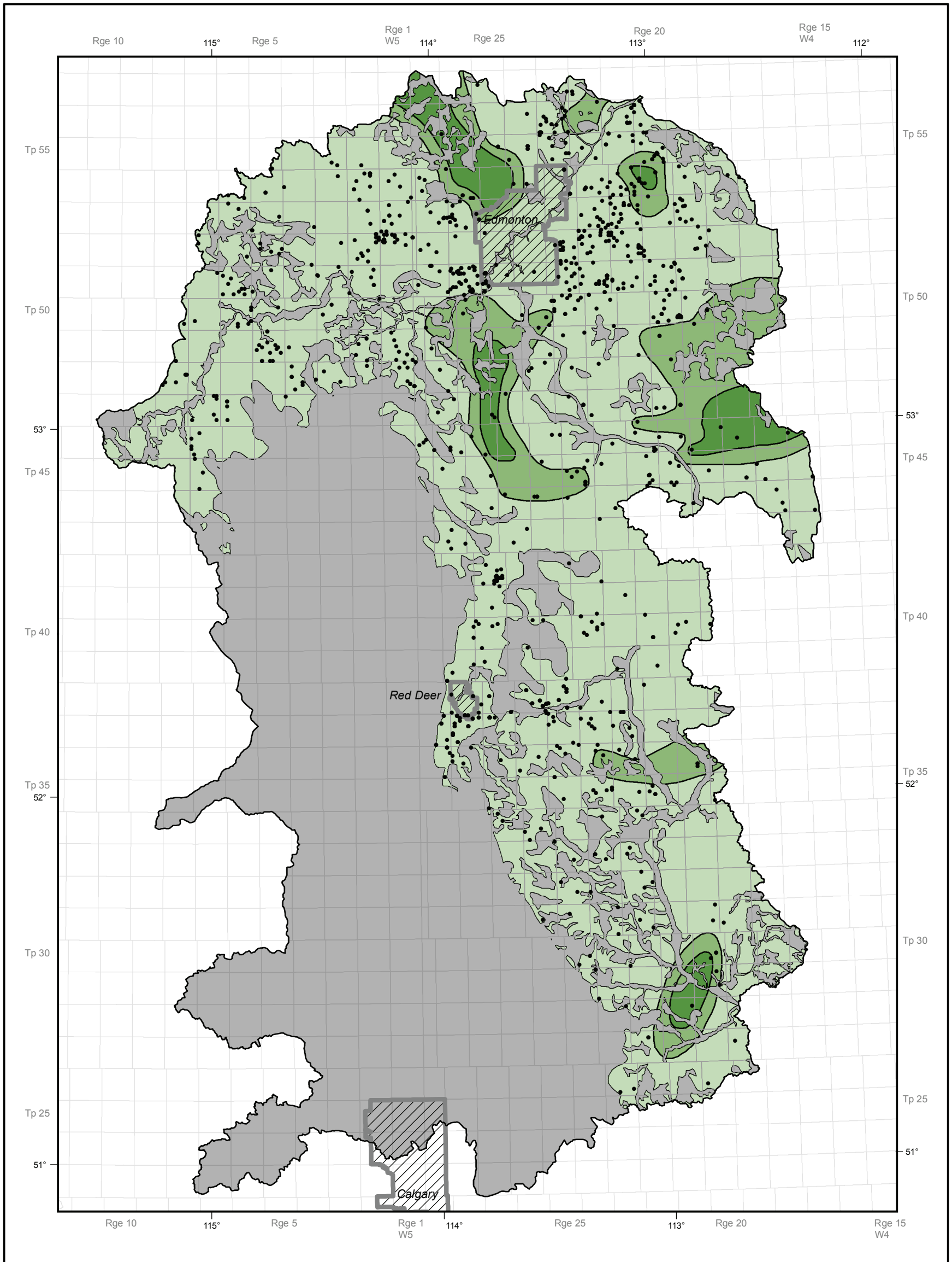
Figure 7. Ranges of chloride concentration in fresh groundwater in the surficial sediments aquifer.
