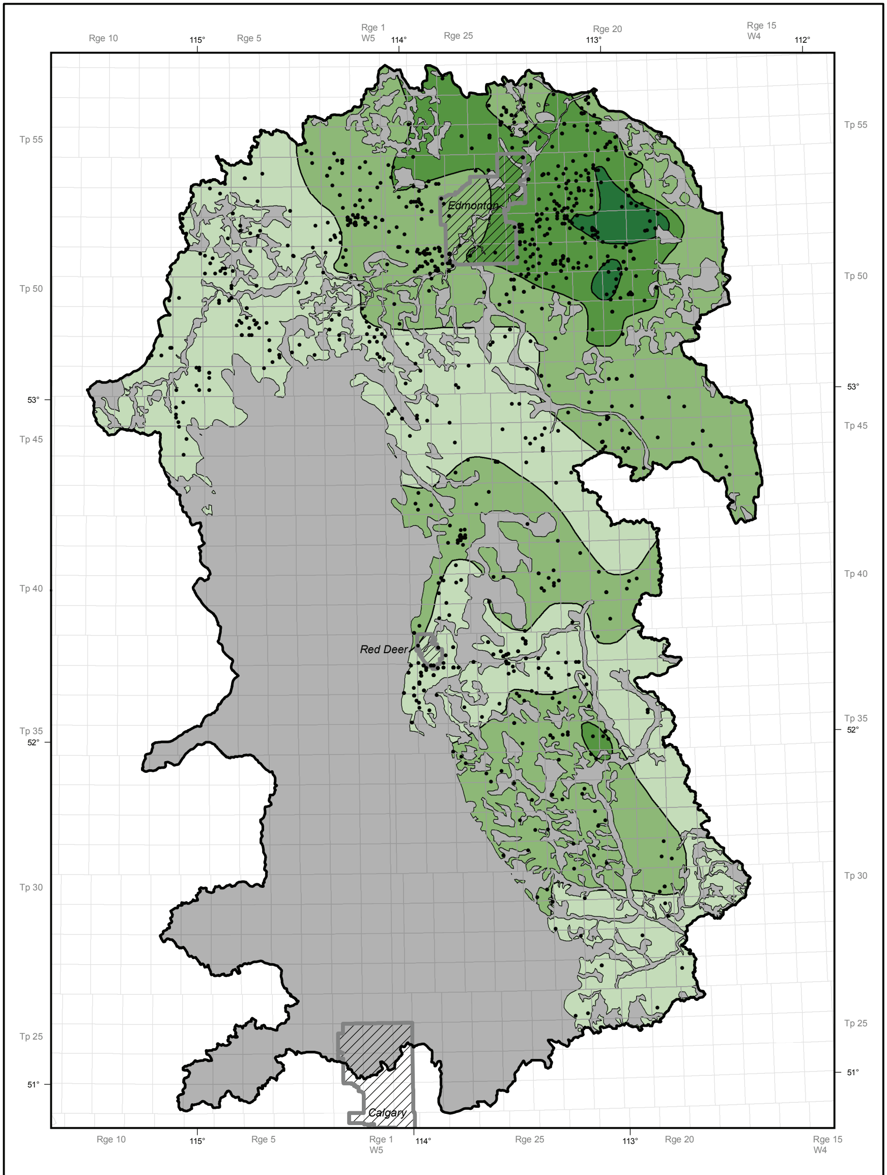
Figure 6. Ranges of potassium concentration in fresh groundwater in the surficial sediments aquifer.
