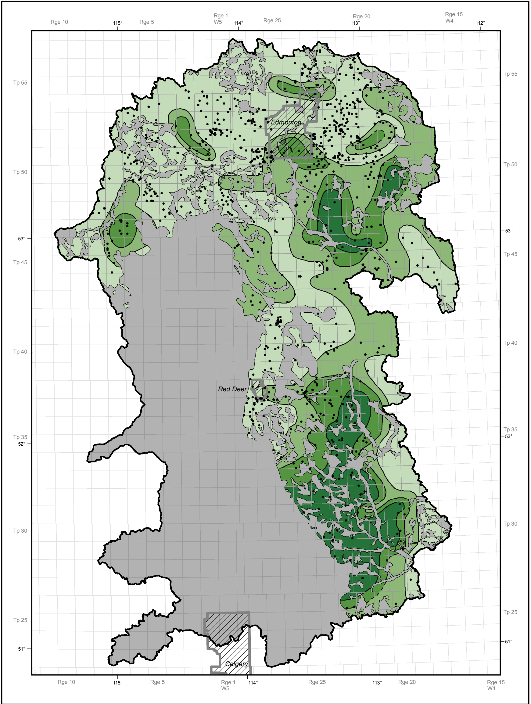
Figure 8. Ranges of sulphate concentration in fresh groundwater in the surficial sediments aquifer.
