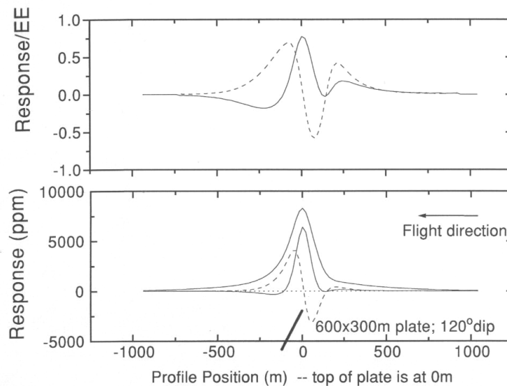
Fig. 5 (Bottom) same as Figure 4, except the plate is now dipping at 120°. On the top graph note the down-dip (left) peak on the normalized z-component response is larger than the right peak (c.f. Figure 4).
