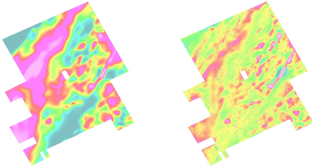
Figure 1. Residual Magnetic Intensity (left) and First Vertical Derivative of Residual Magnetic Intensity (right)
