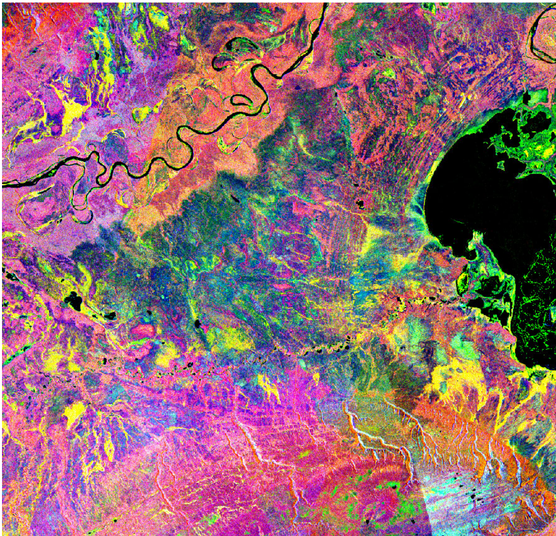
Figure 8. Pseudocolour composite of NTS 84I image dataset of principal component PC1, PC2, PC3 and PC4 (RGB=PC2, PC1, PC3).
