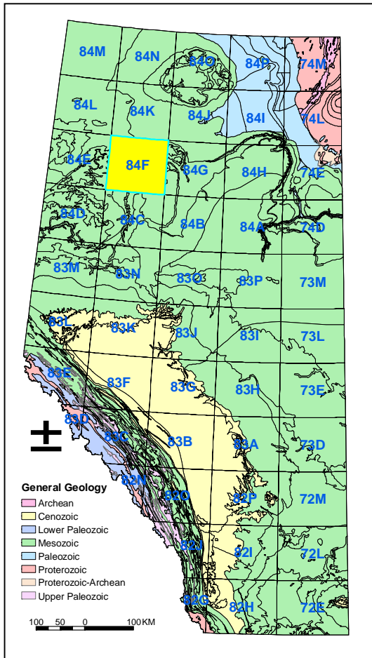
Figure 5. The scenes overlaying NTS 84F.
