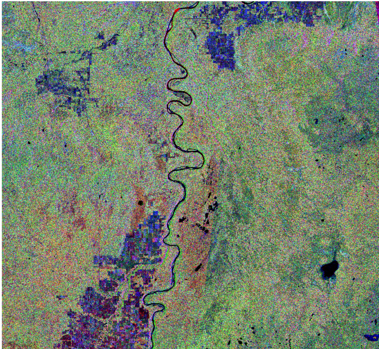
Figure 7. Pseudocolour composite of orthorectified NTS 84F image dataset of Standard Beam Mode S1/S7 ascending/descending beam positions (RGB=S7d, S7a, S1d).
