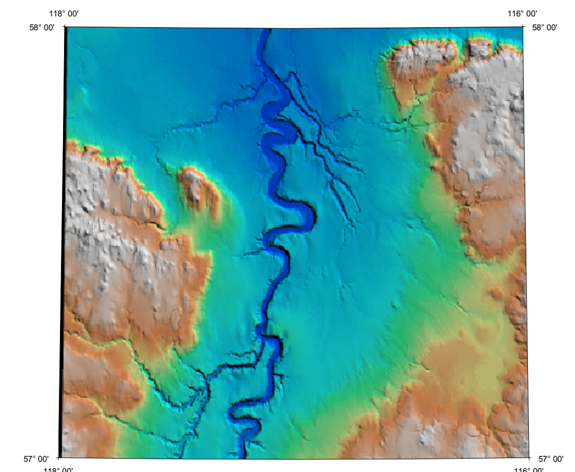
Elevation Map for NTS 84F
