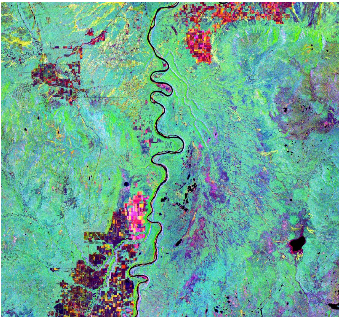
Figure 8. Pseudocolour composite of NTS 84F image dataset of principal component PC1, PC2, PC3 and PC4 (RGB=PC2, PC1, PC3).
