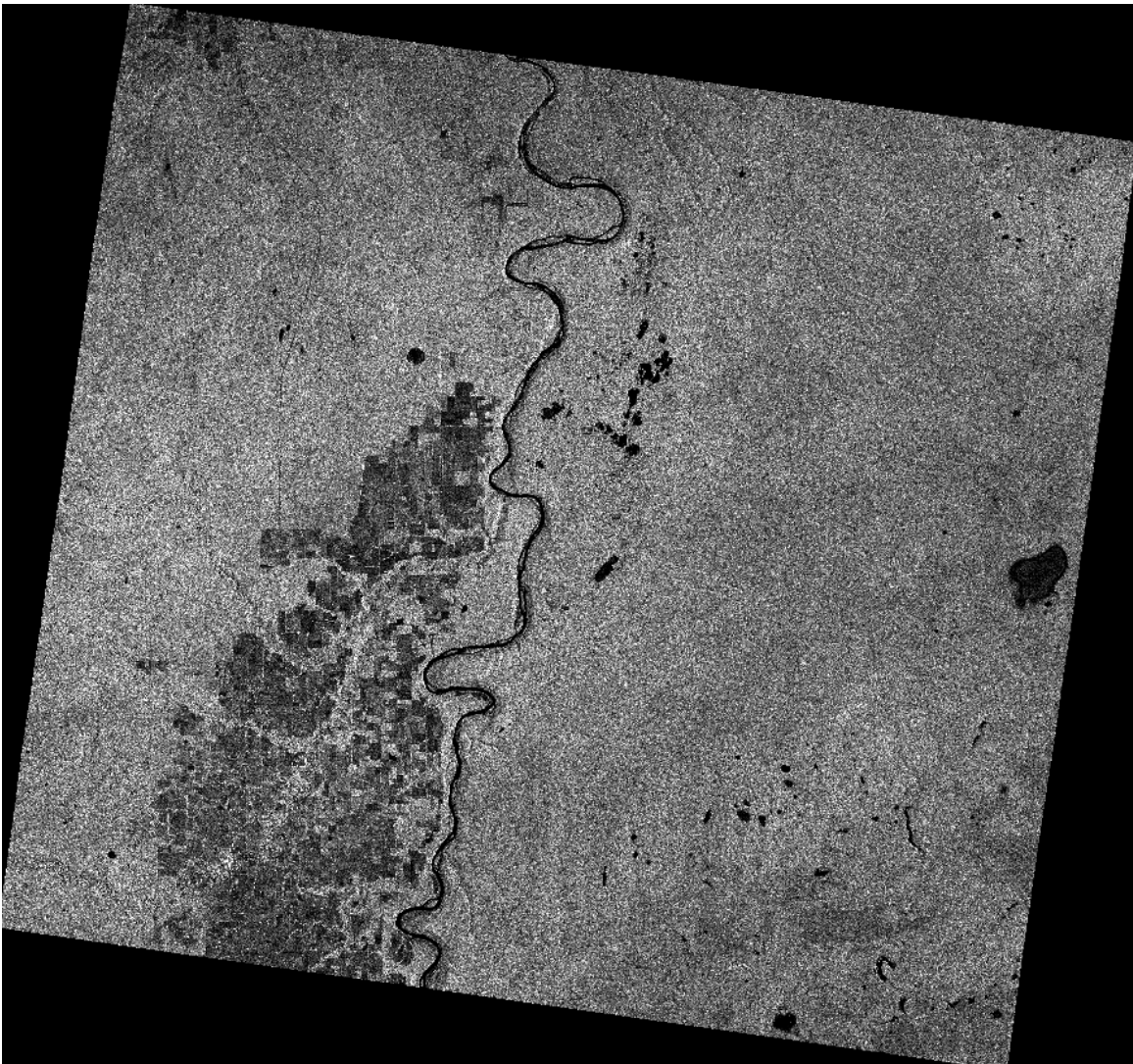
Figure 6. One of the orthorectified scene images used for tiling the NTS 84F dataset: scene MO200096 of Standard Beam Mode 7 descending.
