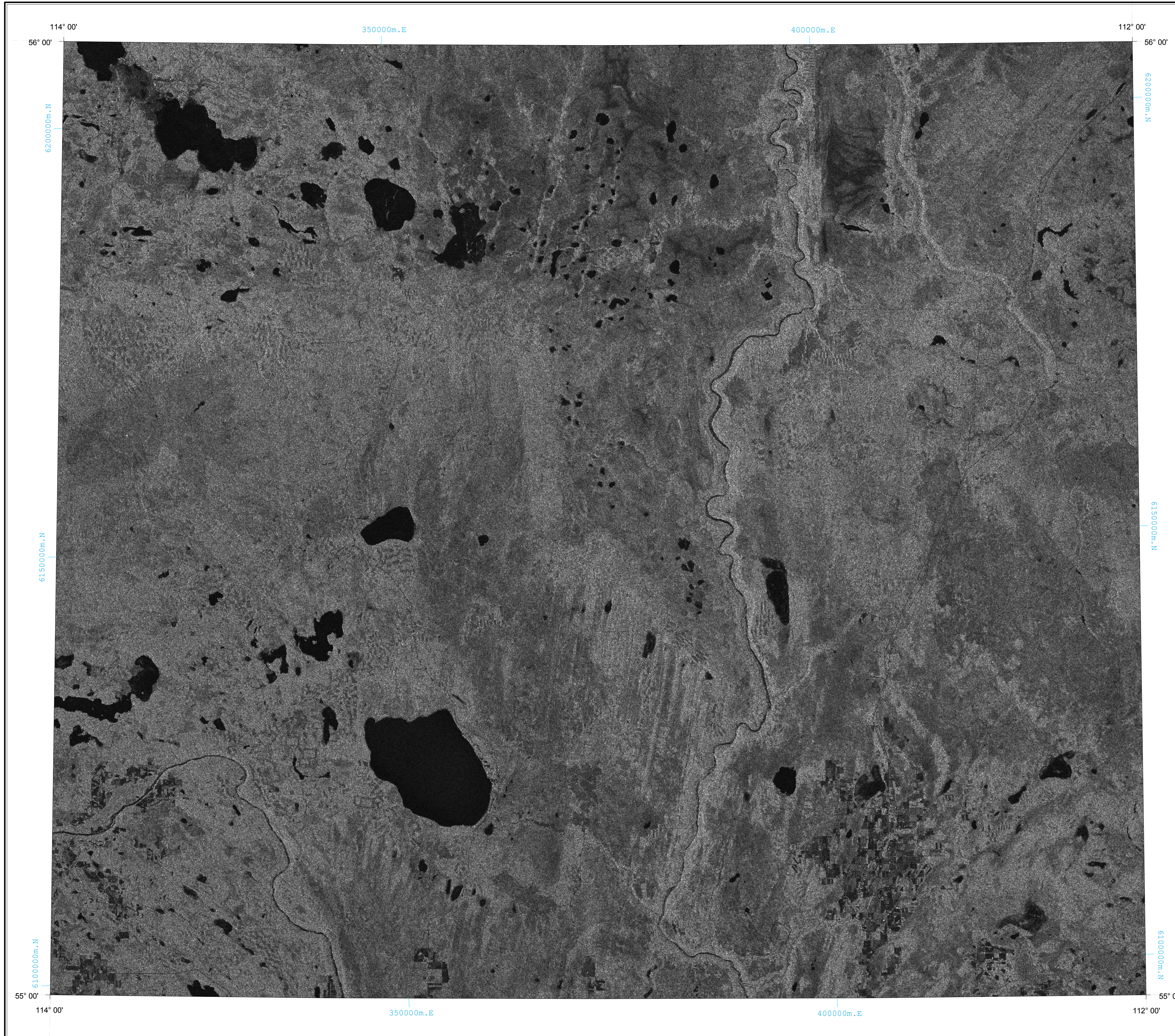
Geo-Note 2003-19, Figure 11
