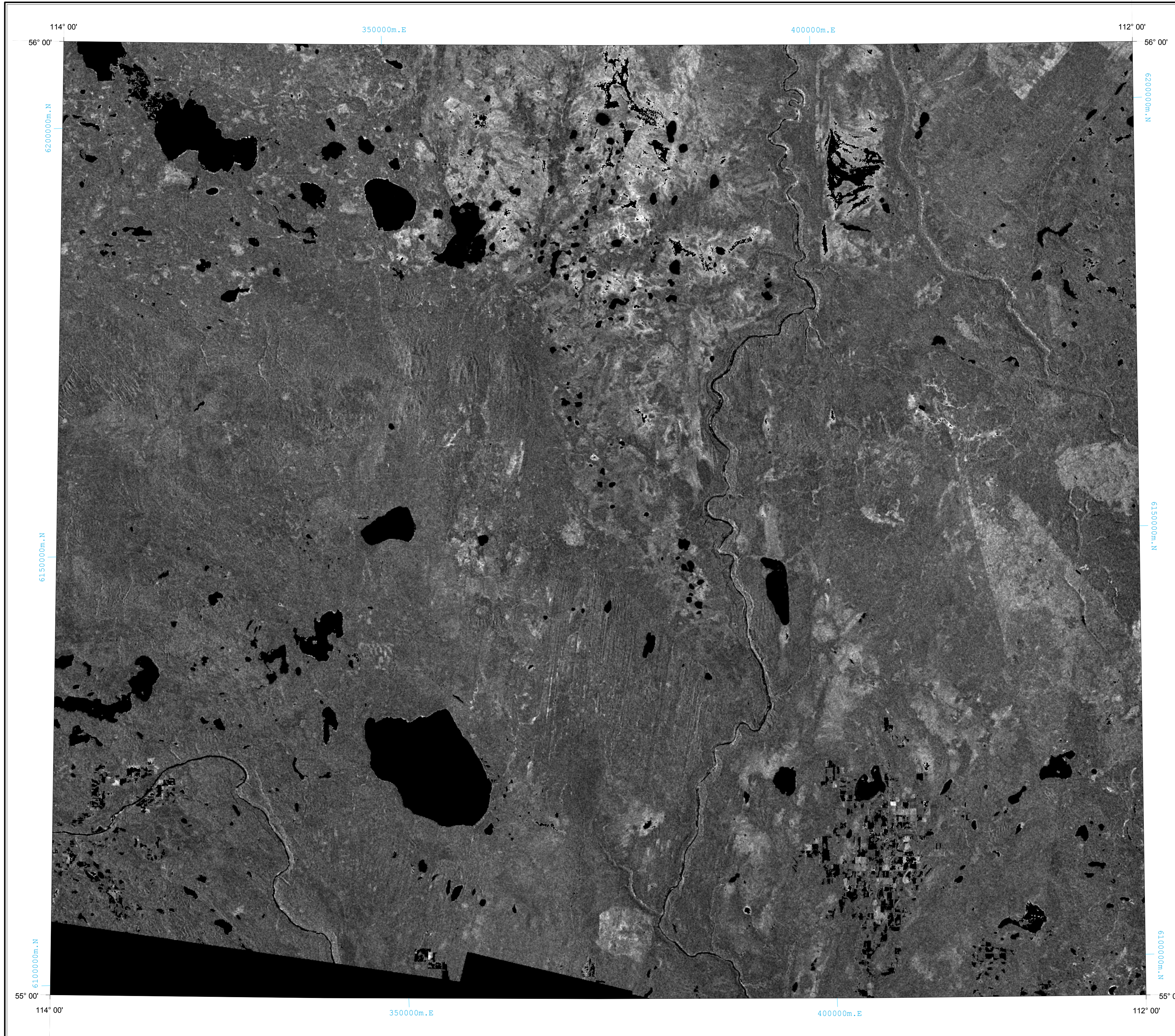
Geo-Note 2003-19, Figure 14
