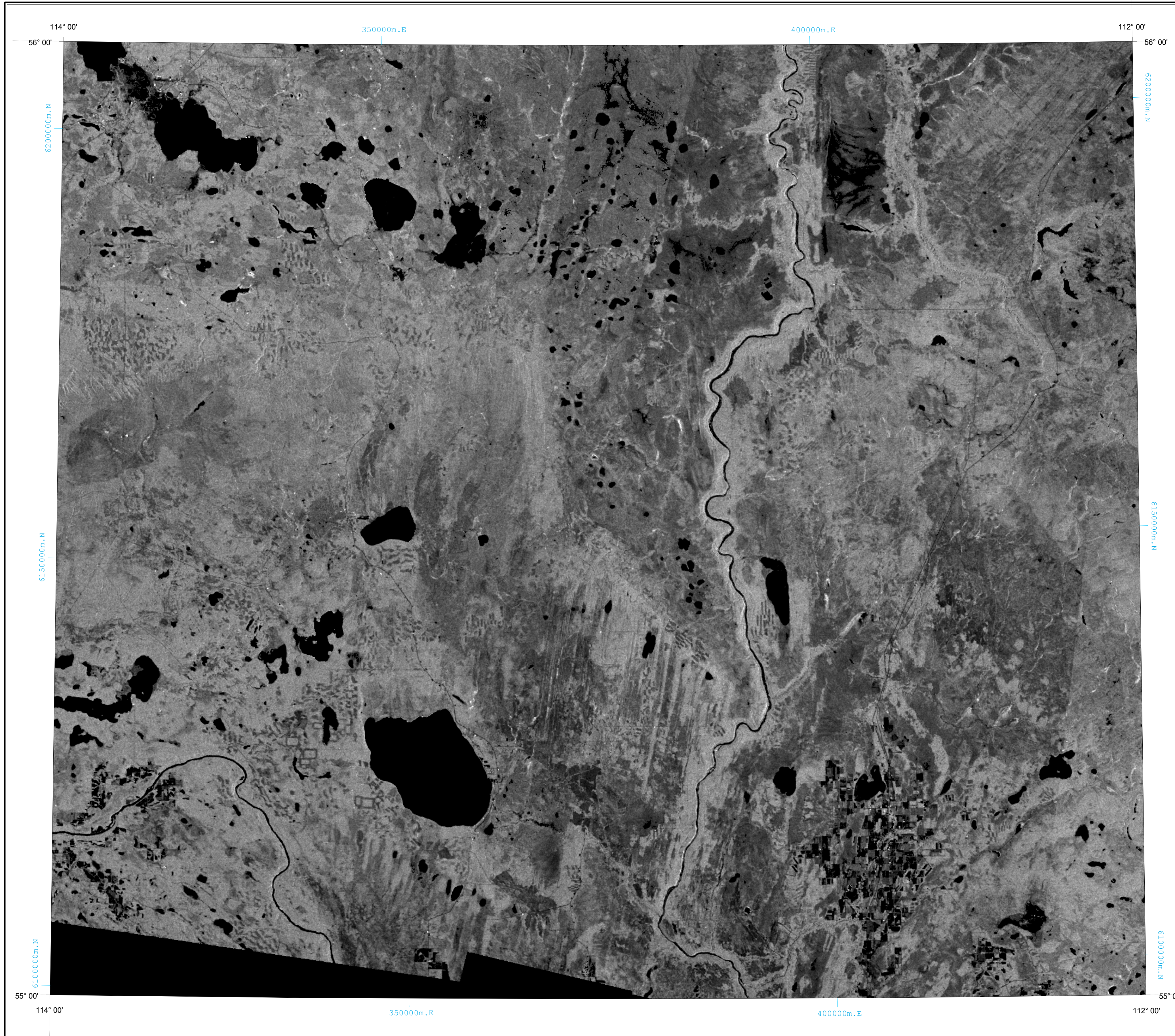
Geo-Note 2003-19, Figure 13
